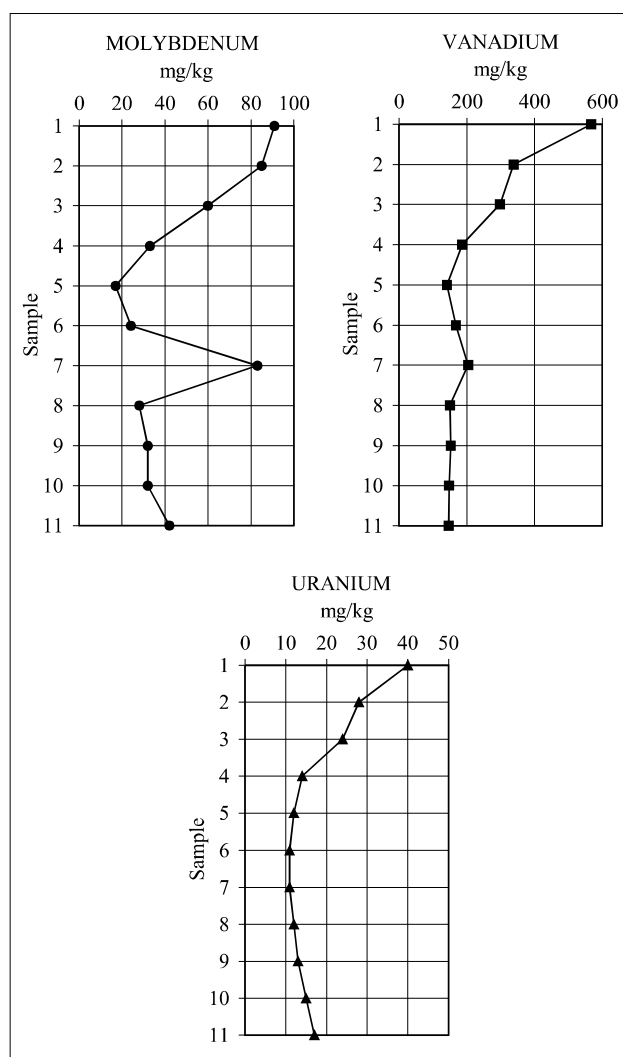
Fig. 27 Distribution of Mo, U and V along along the profile in the Trijezerca quarry.
