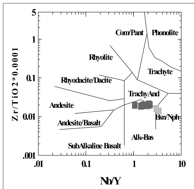
Fig. 29 Diagram after WINCHESTER & FLOYD (1977) for greenish-grey clays from Tri jezerca quarry (dark grey) and insoluble residue of limestone from the Tri jezerca quarry and Kanfanar quarry (light grey).
