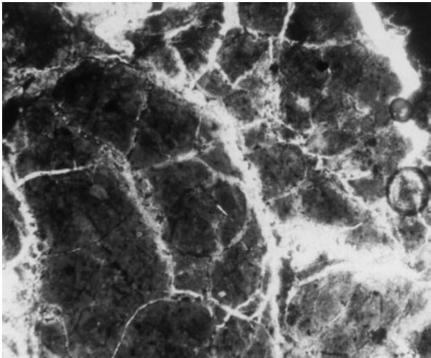
Fig. 33 Fissure microstructure. Basic mass consists of micromass only. Novigrad profile. Depth=145 cm. Length of photograph=7.5 mm.
