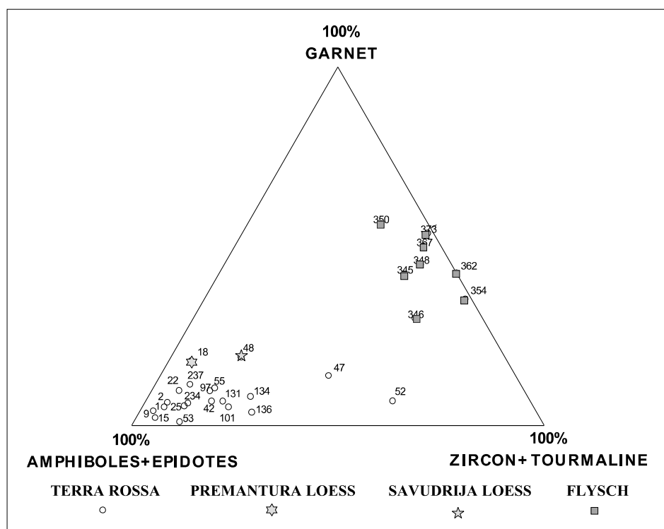
Fig. 38 Relationship between the composition of the selected heavy minerals in terra rossa , loess and flysch. Data for terra rossa and loess from DURN (1996), data for flysch from MAGDALENIĆ (1972).
