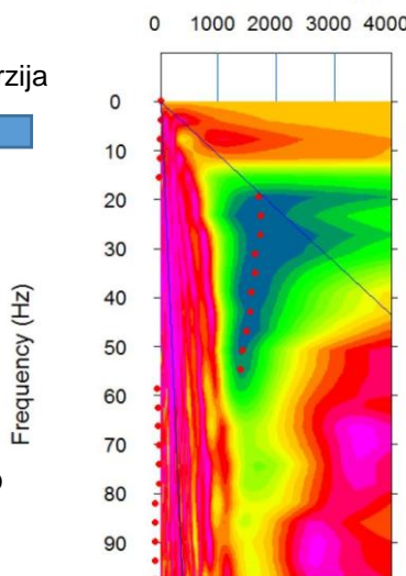
Disperzijska krivulja Source = 47.0m Phase velocity (m/sec)
