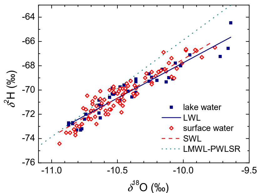
Figure 15. A relation of \delta^2\text{H} vs. \delta^{18}\text{O} for the surface and lake waters at the Plitvice Lakes, 2011–2014. SWL and LWL are shown (Table 4), as well as \text{LMWL-PWLSR} for the Plitvice Lakes.
