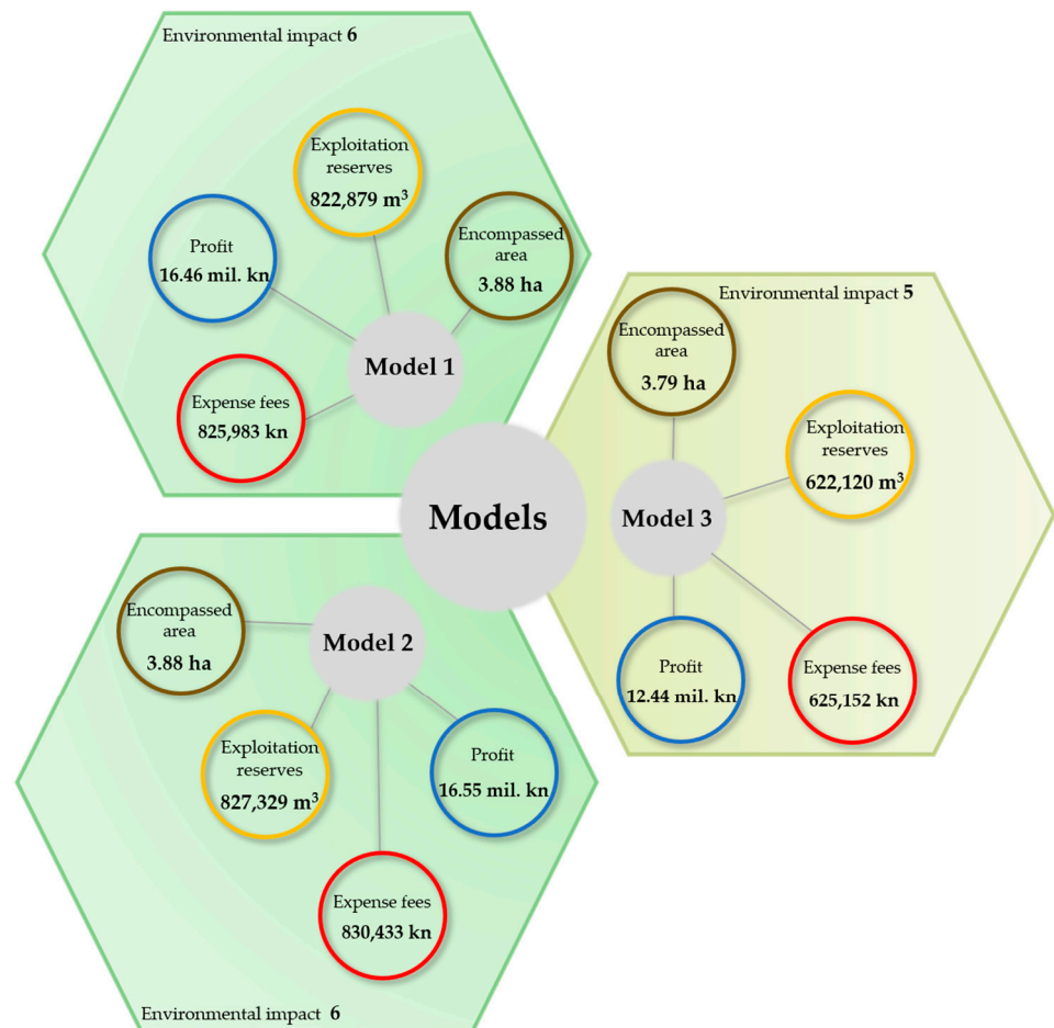
Figure 4. Models of final quarry contours with overview of selected evaluation criteria.
