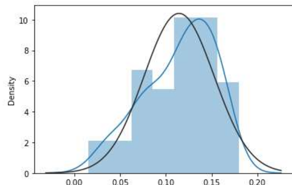
log-normalna (lognorm)
