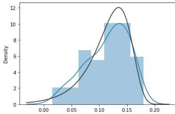
log-gamma (loggamma)
