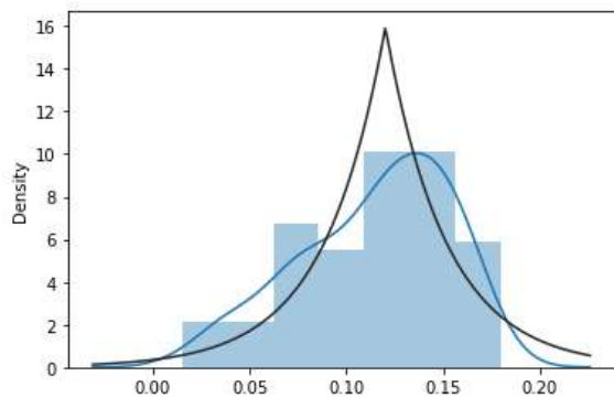
Laplaceova (Laplace)
