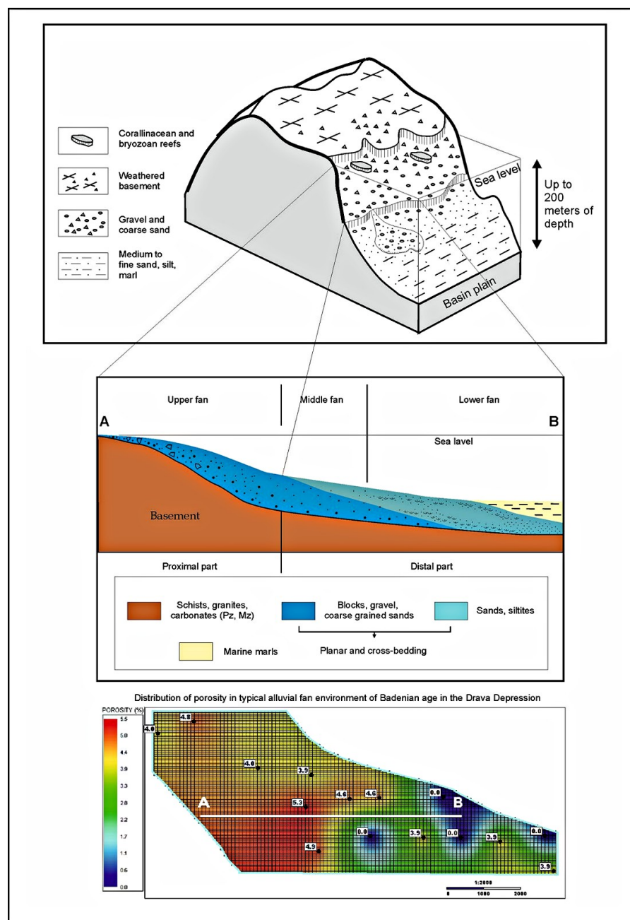
Figure 9. A typical Early Badenian depositional environment, with clinoform structures, reconstructed by [80], based upon the data from the Drava Depression (Stari Gradac Structure).
