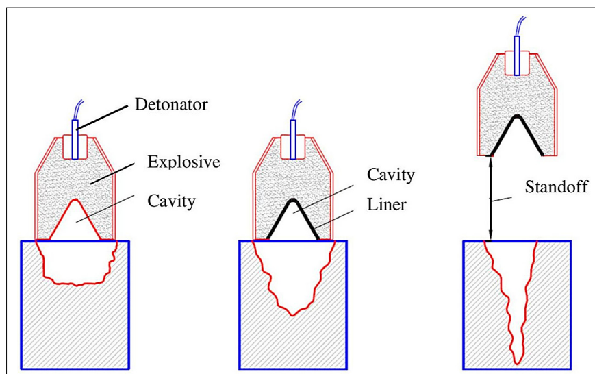
Figure 1: Principle of shaped charges
