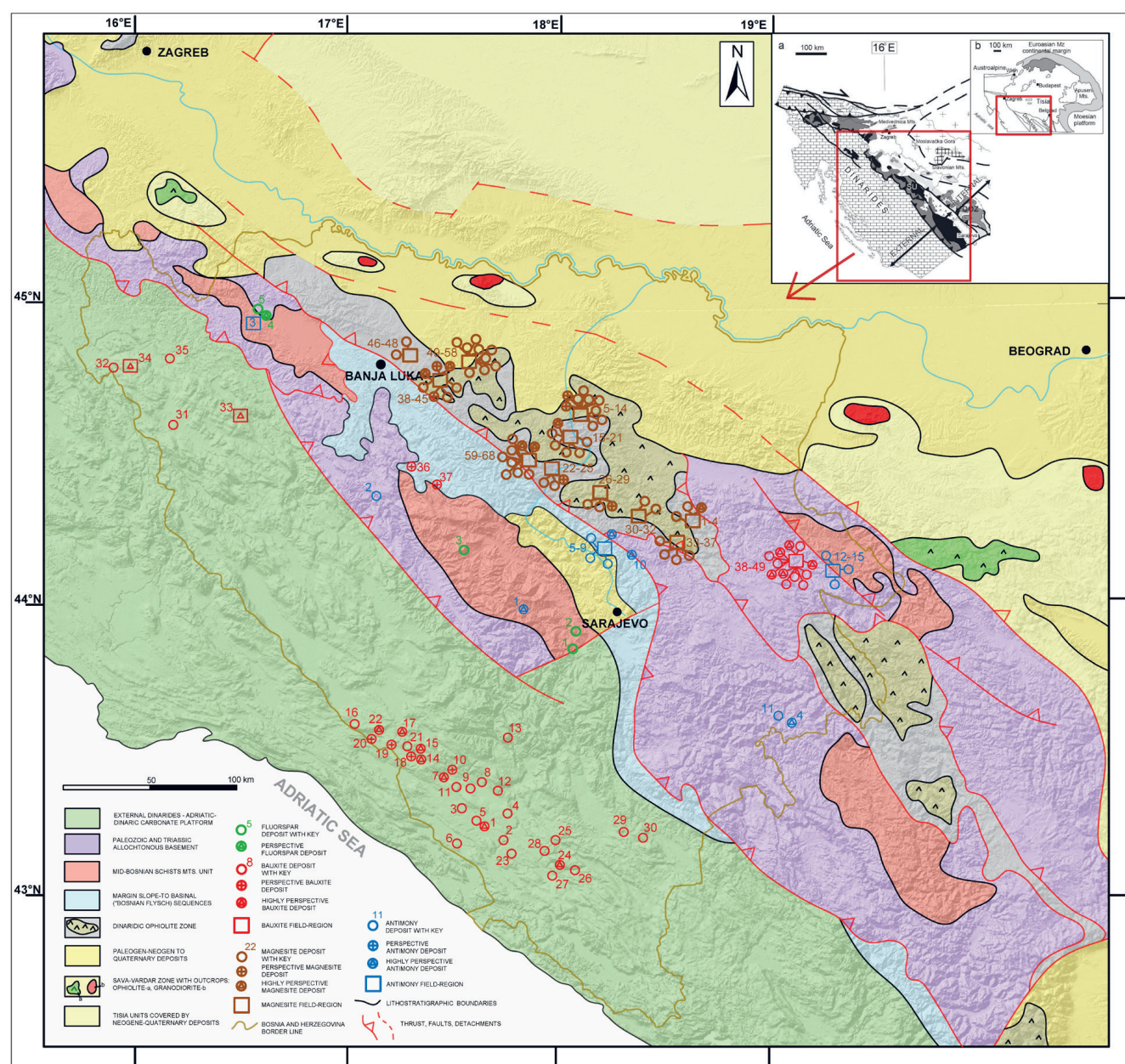
Figure 1. a. Geological scheme of studied area modified after PAMIĆ (1998), TOMLJENOVIC (2008) and PALINKAŠ (2008) with distribution of deposits and occurrences and corresponding keys-numbers linked to Appendix 2, Tables 1-4; b. Regional geological setting according to PAMIĆ (1998) with emplacement (red bound-ed) of studied area.
