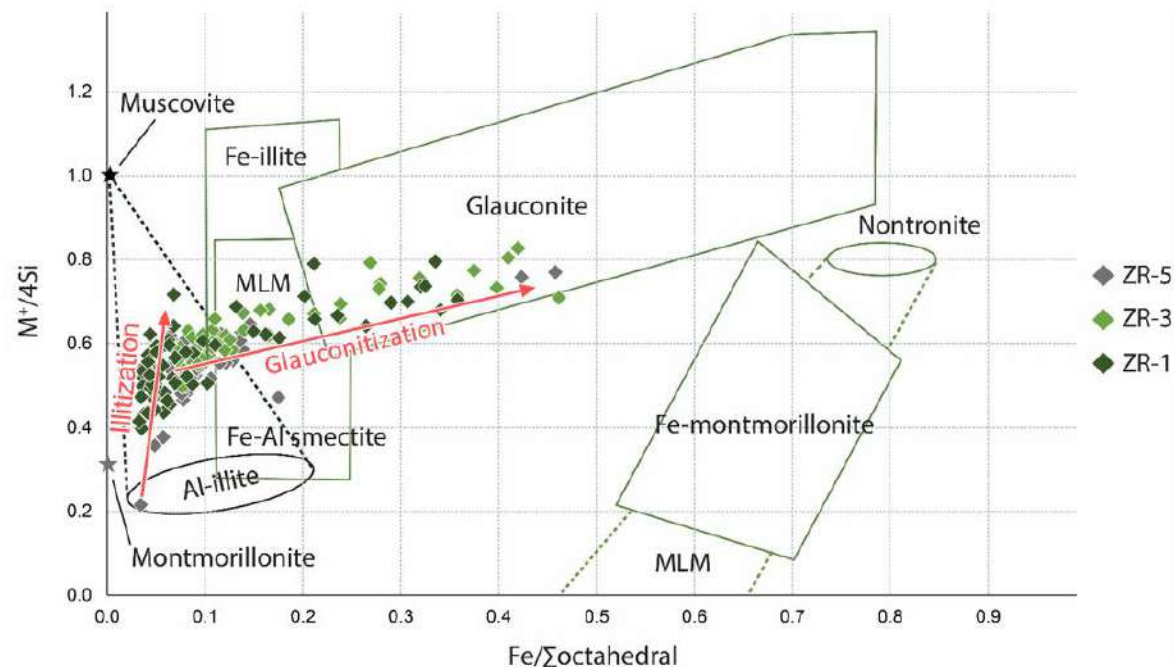
Figure 14. M^{+}/4Si vs. Fe/\Sigma_{oct} plot on which the EDS points measured in ZR-1, ZR-3 and ZR-5 samples have been plotted. Green fields represent data from Meunier and El Albani 2007, while the black fields and stars represent data from Baldernann et al 2014; MLM – mixed layered mineral.
