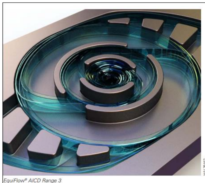
Figure 2-7. Autonomous inflow control device Equi Flow by Haliburton
