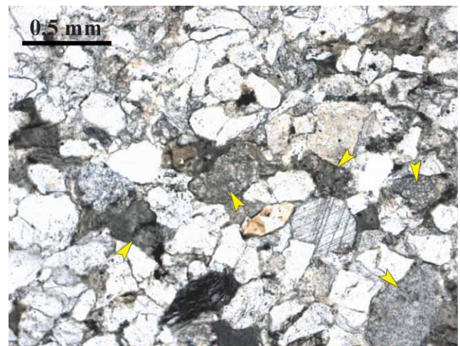
Figure 9: Devitrified volcanic particles in the sandstone showing faint porphyric structure (arrows) and altered feldspars. Stained with Alizarin and K-ferricyanide. Microphotograph; plane polarised light.
