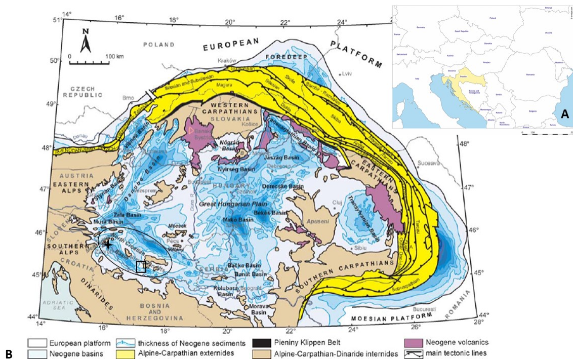
Figure 1: Pannonian Basin System (after Kováč et al., 2007). A) Geographical position of Croatia, coloured in yellow (after https://d-maps.com/carte.php?num_car=2242&lang=en ). B) Pannonian Basin System. Marked area is the location of the Croatian part of the Pannonian Basin System. Four-point star marks the location of Zagreb, capital of Croatia. Rectangular marks the investigated area of the western slopes of the Psunj Mt.
