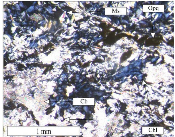
Figure 5–11. Chlorite, muscovite, carbonate mineral and opaque mineral in the Quartz–chlorite–actinolite schist, sample ES 10F–1.
