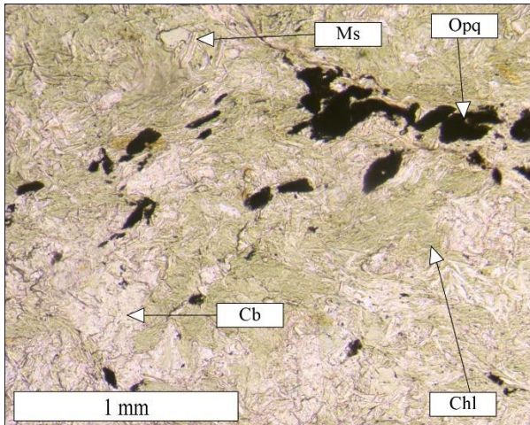
Figure 5–11. Chlorite, muscovite, carbonate mineral and opaque mineral in the Quartz–chlorite–actinolite schist, sample ES 10F–1.
