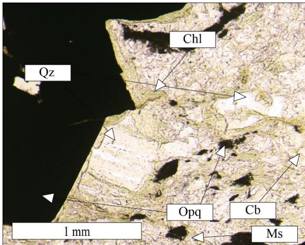
Figure 5–10. Pre-cinematic opaque porphyroblast with pressure shadow of fibrous quartz, chlorite, carbonate mineral and muscovite in the quartz–chlorite–actinolite schist, sample ES 10F–1.
