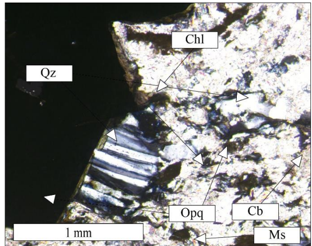
Figure 5–10. Pre-cinematic opaque porphyroblast with pressure shadow of fibrous quartz, chlorite, carbonate mineral and muscovite in the quartz–chlorite–actinolite schist, sample ES 10F–1.
