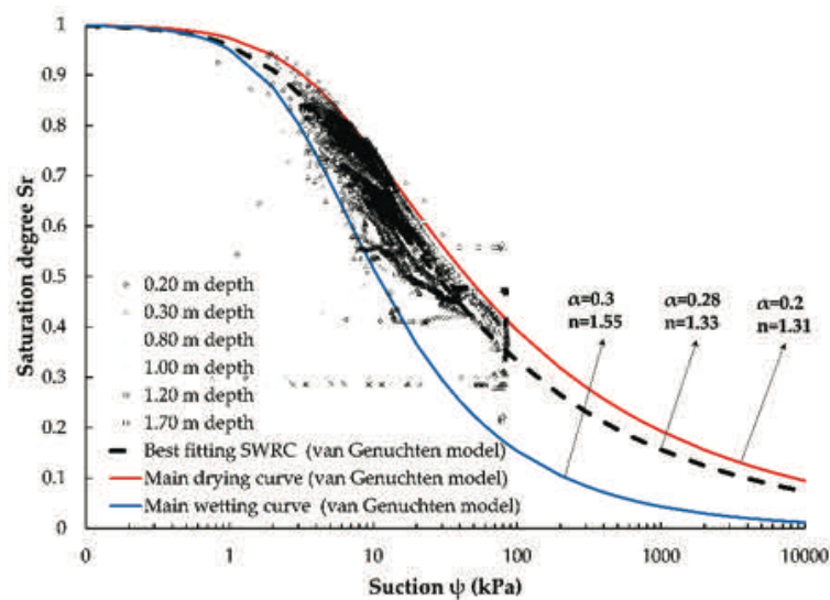
Figure 3 Pairs of suction and saturation degree values, the curve identified by their interpolation, and the main imbibition and drying curves obtained from a laboratory test.
