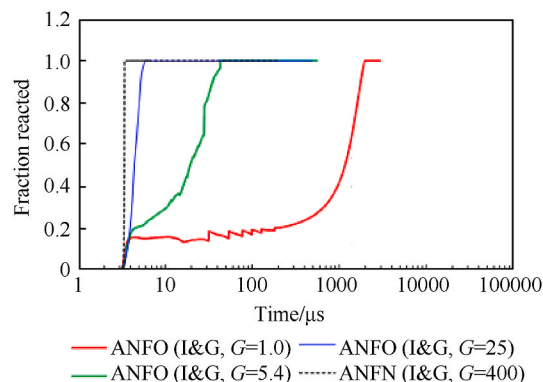
Fig. 8. Fraction reacted vs. time profiles for ANFO charges as a function of reaction rate constant G .
