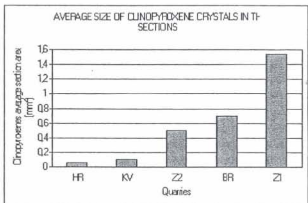
Fig. 2. Average size of main mineral constituents of tested aggregates, measured in thin sections: a – average length of plagioclase crystals, b – average section area of clinopyroxene crystals. (Legend: BR – Brensborg, ZI – Žeravanjska 1, ZZ – Žeravanjska 2, KV – Kraljev Vrh, HR – Hruškovec)
