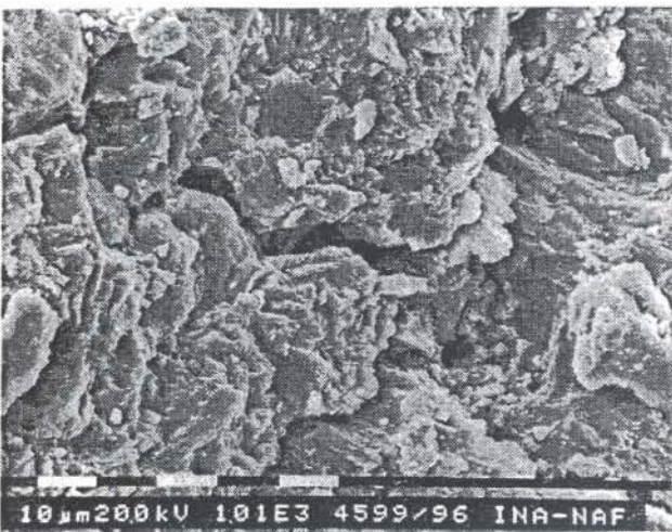
Fig. 3. Scanning electron micrographs of tested samples: a – microfractures in diabase sample Brensbreg are sparse and microblocks are formed only sporadically, b – microfractures in diabase sample Žervanjska 1 are very sparse and isolated, so microblocks are not formed, c – microfractures in diabase sample Žervanjska 2 are sparse and isolated, so microblocks are not formed, d – microfractures in diabase sample Hruškovec are sparse and microblocks are formed only sporadically (Tomašić et al., 1997), e – microfractures in andesite sample Fužinski Benkovac are abundant, clearly visible and intertwined, so numerous microblocks are formed (Tomašić et al., 1997).
