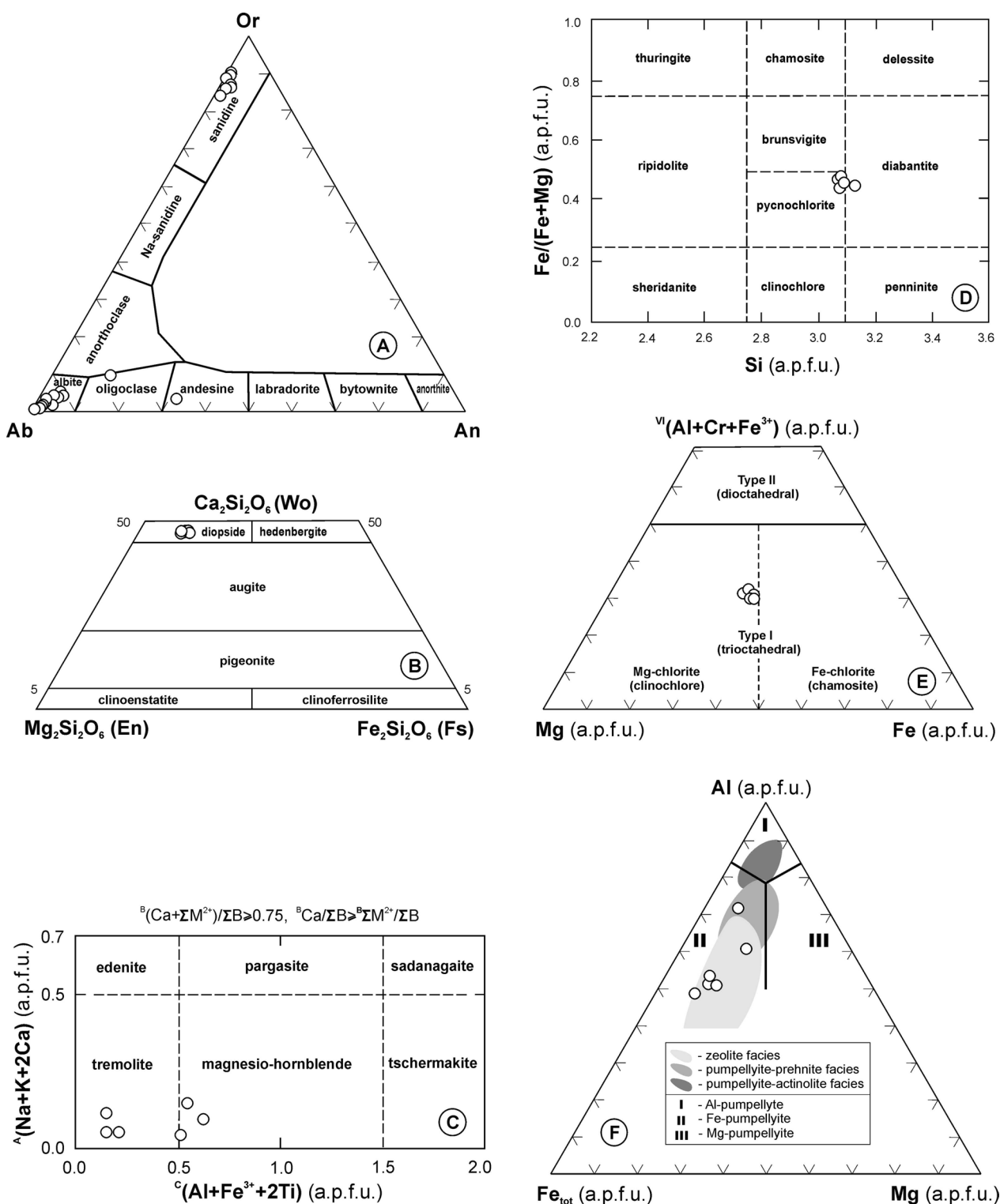
Fig. 4 Classification diagrams for A feldspar [Ab – An – Or plot; Deer et al., 1992, page 2; Dana et al., 1993, page 532], B pyroxene [En – Wo – Fs ( \text{Mg}_2\text{Si}_2\text{O}_6 - \text{Ca}_2\text{Si}_2\text{O}_6 - \text{Fe}_2\text{Si}_2\text{O}_6 ) plot; Morimoto, 1988] C calcium amphibole [ ^A(\text{Na} + \text{K} + 2\text{Ca}) - ^C(\text{Al} + \text{Fe}^{3+} + 2\text{Ti}) plot; Hawthorne et al., 2012], D-E chlorite [ ^{\text{VI}}(\text{Al} + \text{Cr} + \text{Fe}^{3+}) - \text{Si} plot (after Hey, 1954 adapted to Sun et al., 2019); Mg – Fe – ^{\text{VI}}(\text{Al} + \text{Cr} + \text{Fe}^{3+}) plot (Zane & Weiss, 1998)], F pumpellyite [ \text{Fe}_{\text{tot}} - \text{Mg} - \text{Al} plot (adapted after Passaglia & Gottardi, 1973; Coombs et al., 1976)] from the basaltic volcanoclastics from Mt. Ivanščica. The compositional fields of pumpellyite from the East Taiwan Ophiolite (zeolite facies), the Olympic Peninsula (prehnite–pumpellyite facies) and the Taveyannaz Formation (upper prehnite–pumpellyite and pumpellyite–actinolite facies) were taken from Mével (1981), Coombs et al. (1976) and Rahn et al. (1994)
