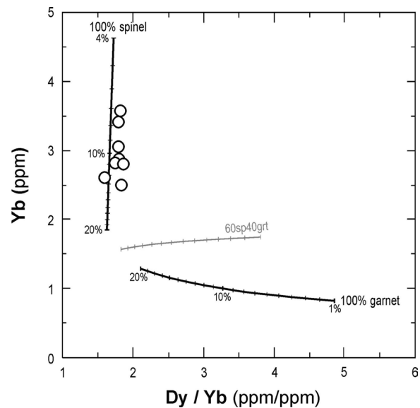
Fig. 11 Yb – Dy/Yb diagram for the basaltic volcanoclastics from Mt. Ivanščica. Partial melting curves are shown for the non-modal batch melting of spinel and garnet ilherzolite sources, starting from a Primitive Mantle (PM; McDonough & Frey, 1989) material. Mineral and melt modes for spinel and garnet-ilherzolite source: \text{Ol}_{0.58(0.10)} + \text{Opx}_{0.27(0.27)} + \text{Cpx}_{0.12(0.50)} + \text{Sp}_{0.03(0.13)} (Kinzler, 1997) and \text{Ol}_{0.60(0.05)} + \text{Opx}_{0.21(0.20)} + \text{Cpx}_{0.08(0.30)} + \text{Gt}_{0.12(0.45)} (Walter, 1998), respectively. Italic numbers in parentheses indicate the percentages of each mineral entering the liquid. Partition coefficients are from McKenzie & O'Nions (1991)
