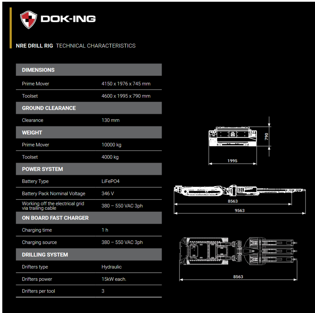
Figure 4-3 NRE Drill Rig (Dok-ing, 2024)
