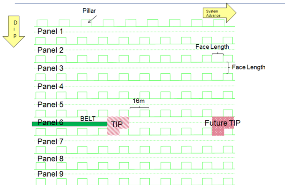
Figure 3-3 Room and pillar mining method (Valicek et al., 2012)
