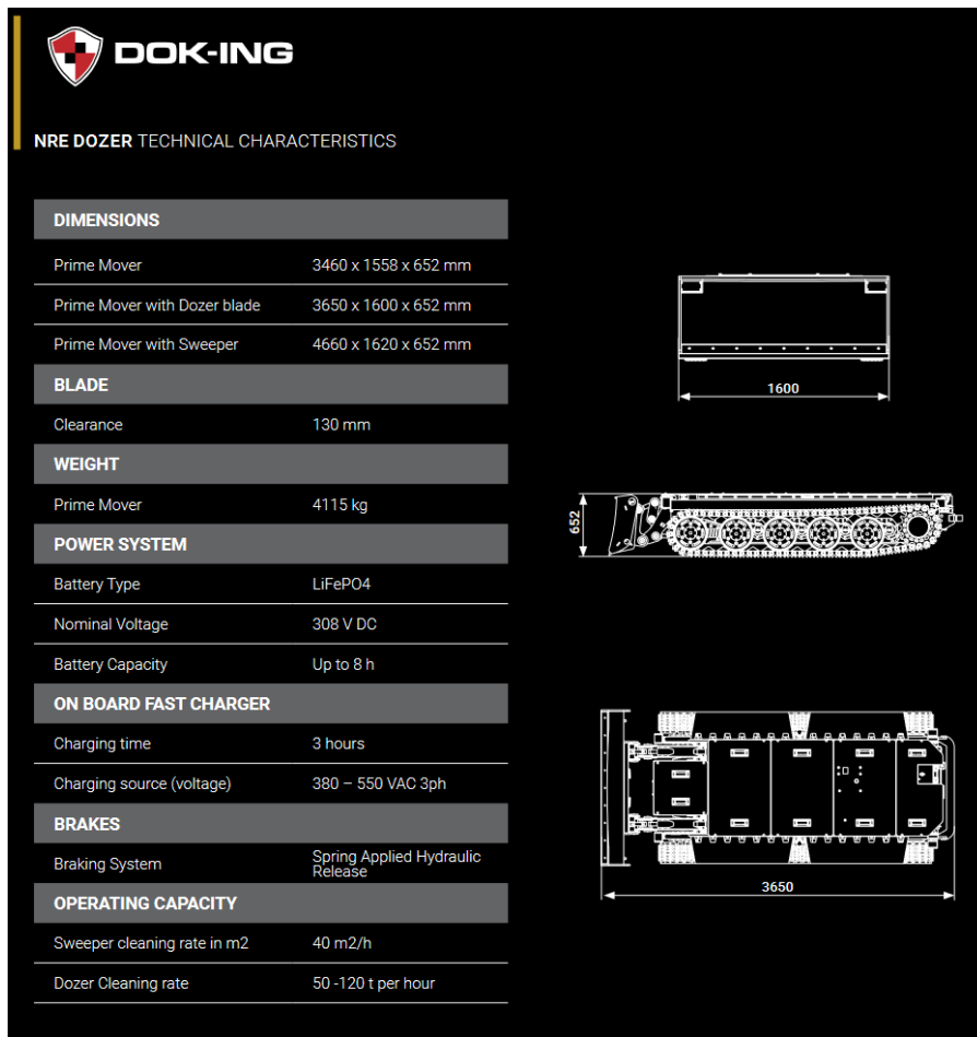
Figure 4-2 NRE Dozer (Dok-ing, 2024)
