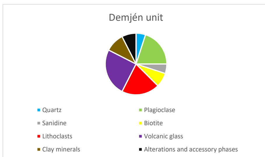
Figure 5-8. Mineral, lithoclast, and volcanic glass distribution in samples from the Demjén unit
