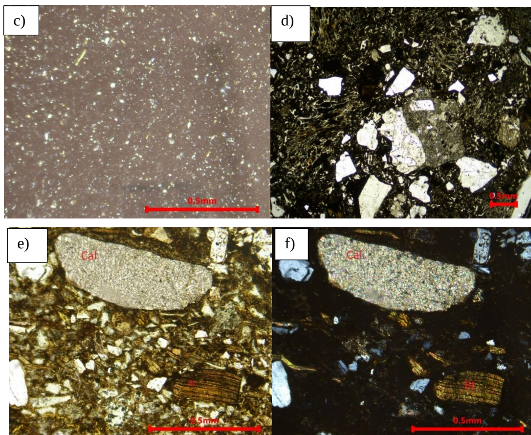
Figure 5-7. a) Plagioclase and biotite in sample Dem-30, N; b) Zoned plagioclase and biotite in sample Dem-30, N+, c) Dark volcanic glass particles in sample KMJ-01, N+; d) Lithoclast in sample Dem-9_E/6, N; e) Calcite pseudomorphosis after feldspar in sample KMJ-02, N; f) Calcite pseudomorphosis after feldspar in sample KMJ-02, N+
