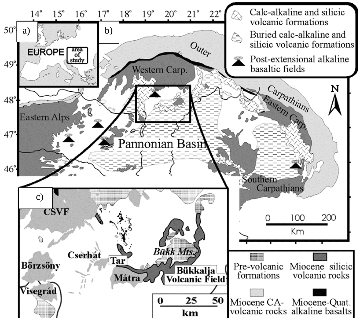
Figure 3-3. 3. Location of the BFV a) in Europe; b) in the Carpathian-Pannonian region; c) in the Northern Hungary ;Carp—Carpathians,CSVF—Central Slovakia. (Harangi et al, 2005).
