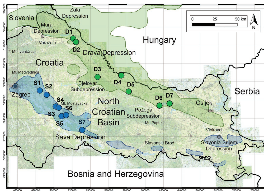
Fig. 3. Position of the North Croatian Basin and locations of exploration wells, which are the subject of this study within the approximate areas of the Sava (S1–S7) and Drava Depression (D1–D7), including neighboring Neogene depressions and sub-depressions.
