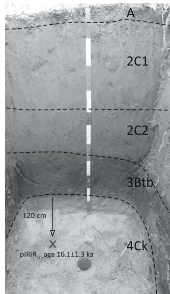
Figure 1. Polygenetic soil profile at the Susak Island (From: DURM et al., 2017).
