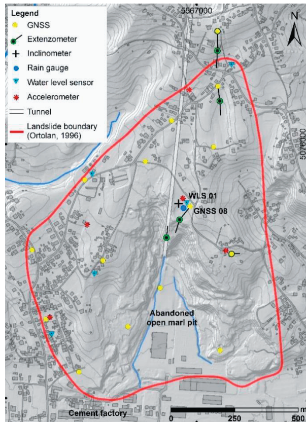
Figure 6. Multiple sensor networks at the Kostanjež landslide (KRKAČ et al. , 2017).
