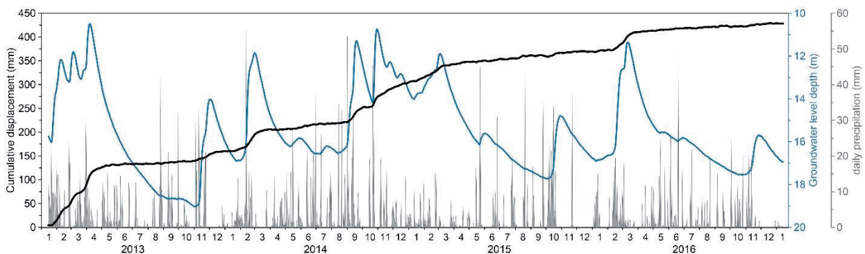
Figure 7. Displacements and groundwater level depths measured at the central monitoring station of the Kostanjež landslide and 1-day antecedent precipitations measured at Zagreb-Grič meteorological station.
