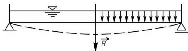
Figure 4. Water load model
