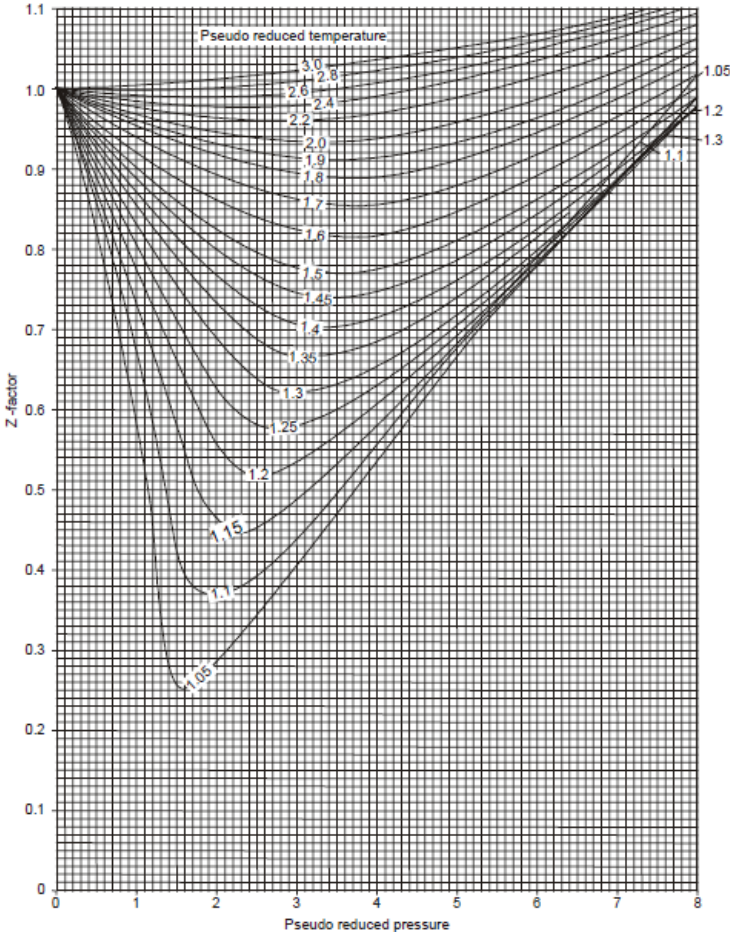
Figure 6-2. Z-factor diagram (Arnold, Stewart, 2008)
