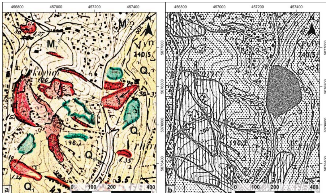
Figure 3: Landslide inventory map from 1979 in scale 1:10,000 (Polak et al., 1979): (a) Lithological map ( Q_{al} – Alluvial deposits; Q_1 – Pleistocene deposits (clay, silt); M_7^z – Upper Pontian deposits (sand, silt)) with landslide polygons (red polygons are active landslides; green polygons are inactive landslides; blue lines are wet areas or lines of periodic superficial flows); (b) Landslide susceptibility map (dotted pattern - conditionally stable slopes; striped pattern - conditionally unstable slopes; black pattern - unstable slopes).
