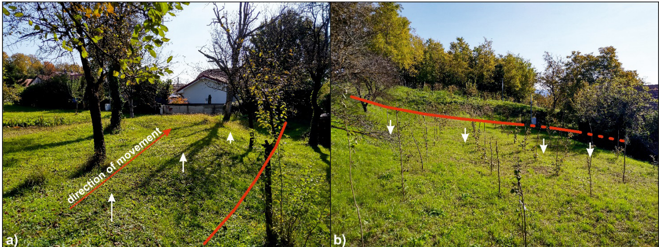
Figure 8: Vertical deformations at the Kostanjek landslide: a) uplift of the material (white arrows) at the western boundary (red line); b) subsidence (white arrows) along the minor scarp (red line) in the eastern part of the landslide
