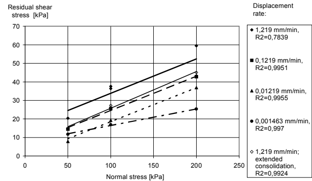
Fig. 5. Residual shear strength envelopes.
