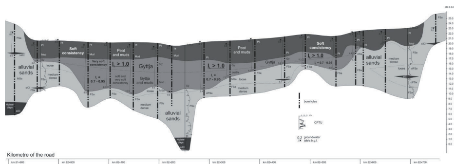
Fig. 4. Verified geological model on cross-section with layers of peat and gyttja on eastern lane of highway (verification of geological model stage II – 2016) [4]
