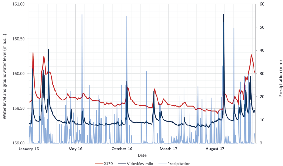
Figure 9. Pluviograph obtained from mean precipitation from meteorological stations compared to the level of the Vidovičev mlin hydrological station and piezometer 2179.
