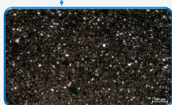
Thin section of archeological ceramic (XP)
