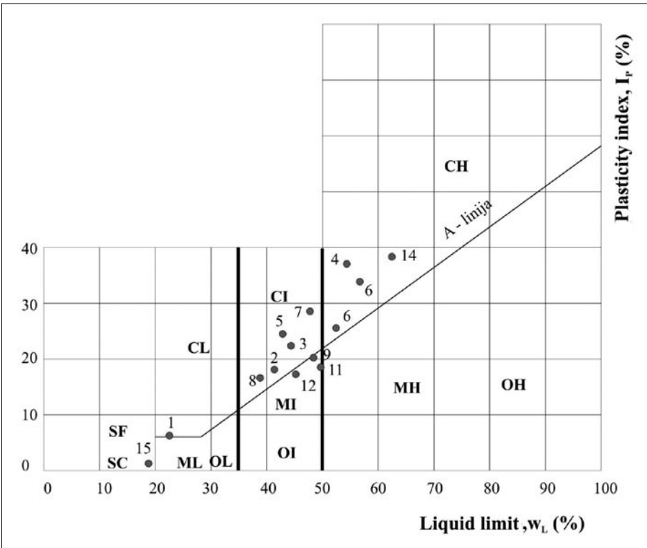
Fig. 19 Plasticity chart.
