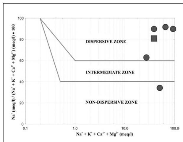
Fig. 23 Cations in the pore water of the flysch samples. Potential dispersivity chart after SHERARD et al. (1976). Stability after pinhole test: rectangle – nondispersive, circle – dispersive.
