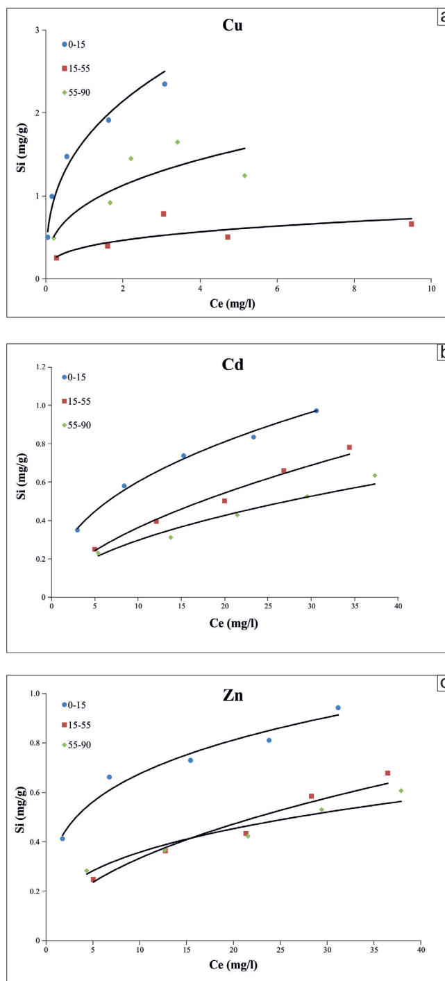
Figure 7. Freundlich sorption isotherms for Profile 4: a) Cu; (b) Cd; (c) Zn.
