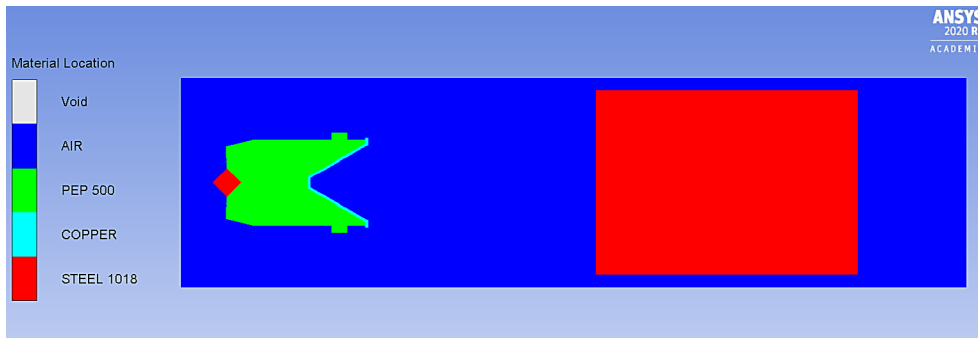
Figure 4: Penetration process modelling
