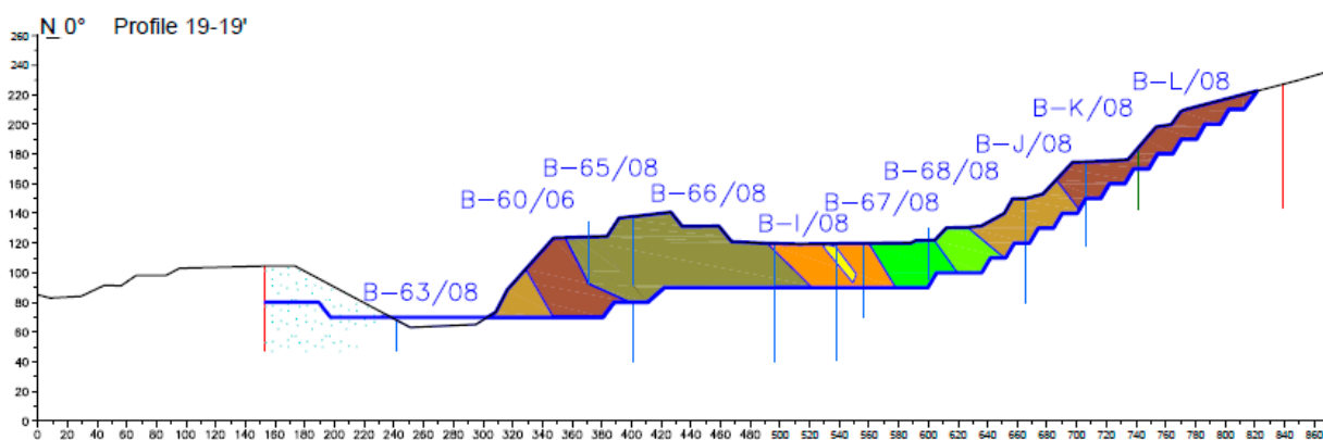
Figure 5. Transversal geological cross-sections 5-5' and 19-19'.
