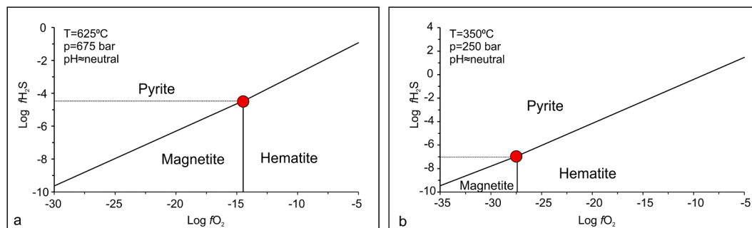
Fig. 16. Stability of hematite, magnetite and pyrite in the \log f_{\text{O}_2} vs. \log f_{\text{H}_2\text{S}} field constructed for a) Ore-forming conditions associated with development of the potassic alteration zone and b) Deposition of the sulfide mineralization in the chlorite alteration zone of the Vršnik ore body, the Bučim porphyry Cu-Au deposit, North Macedonia. The thermodynamical modelling was performed using the SUPCRT model and the associated databases (Johnson et al. 1992).
