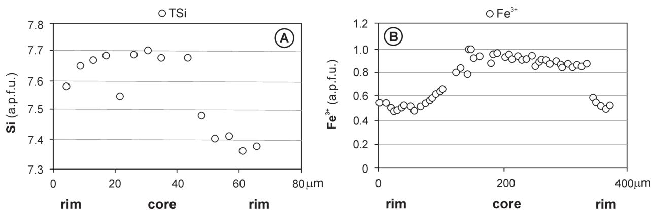
Fig. 7. Chemical profile through the prograde grain of amphibole (A) and epidote (B) in sample Md-4 (Tusti Breg Unit).
