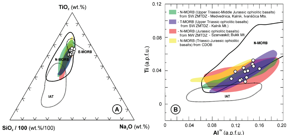
Fig. 14. Discriminant diagram SiO 2 /100–Na 2 O–TiO 2 (A) and Al IV –Ti (B) (simplified after Beccaluva et al. 1989) for clinopyroxene from ortho-greenschists from Mt. Medvednica metamorphic complex. IAT= island-arc tholeiites, E-MORB=enriched mid-ocean ridge basalts, N-MORB=normal mid-ocean ridge basalts. Field of clinopyroxene composition of the Jurassic extrusives from the northeastern part of ZMTDZ (Szarvaskő complex in Mt. Bükk; Balla & Dobretsov 1984) and basalts from CDOB (Lugović et al. 1991) are plotted for correlation constraints.
