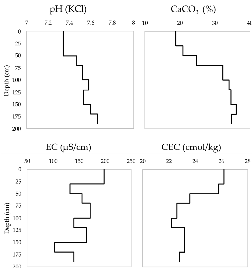
Figure 3. Vertical distribution of pH, EC, CaCO 3 and CEC in the study soil profile.
