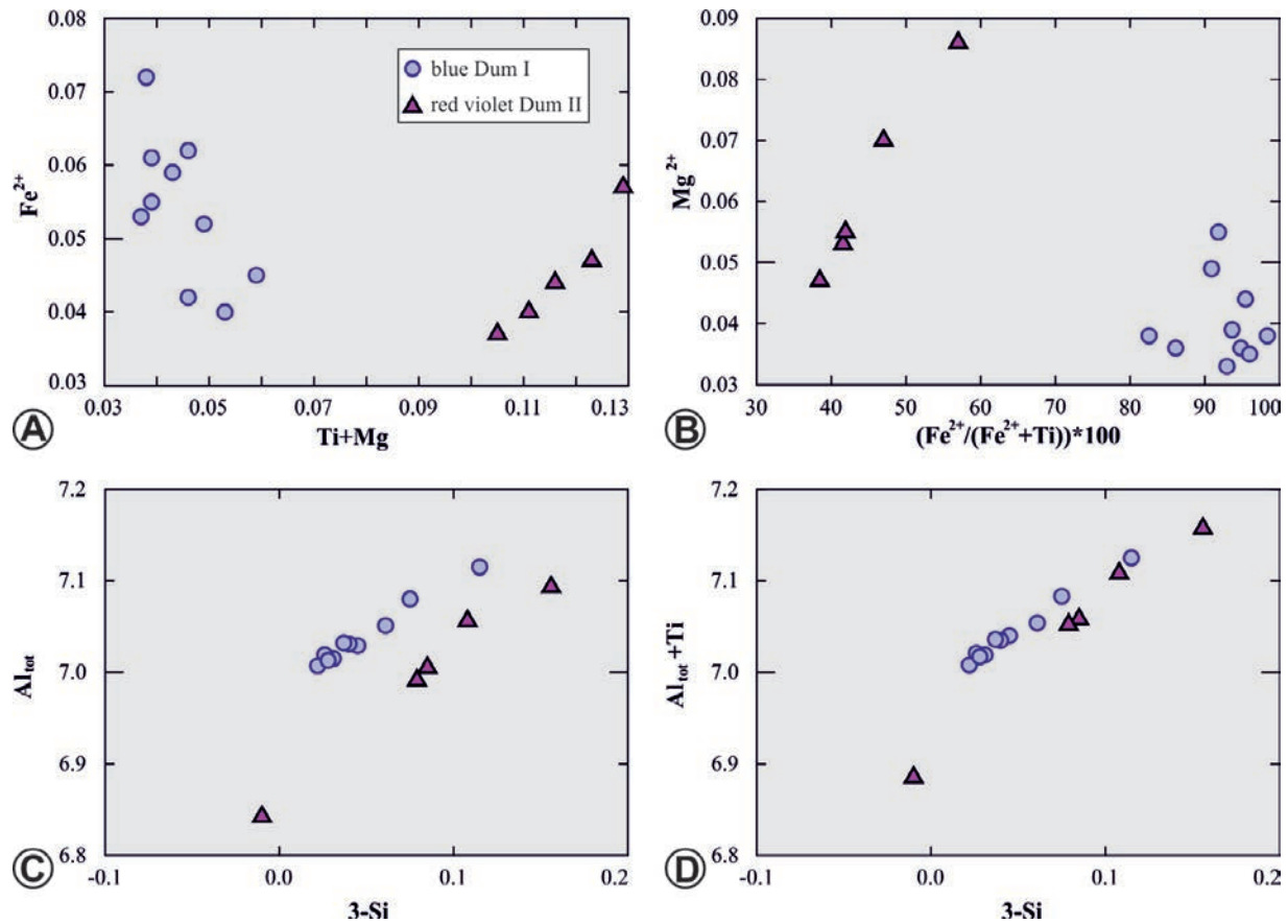
Figure 10. Chemical composition of dumortierite from Mt. Moslavačka Gora. A) \text{Fe}^{2+} vs (\text{Ti}+\text{Mg}) diagram showing a clear positive correlation between \text{Fe}^{2+} and the sum of Ti and Mg in the crystal lattice of red to violet Dum II but a moderately negative correlation for blue Dum I crystals. B) In the \text{Mg}^{2+} vs [\text{Fe}/(\text{Fe}+\text{Ti})]\times 100 ratio diagram, a strong positive correlation is visible for Dum II, whereas Dum I shows a moderately negative correlation. C) In the \text{Al}_{\text{tot}} vs 3-Si diagram, all dumortierite analyses taken together show a badly defined moderately positive correlation ( R^2 = 0.51 ) but when considering Dum I and Dum II separately, a well defined correlation is visible. D) In the \text{Al}_{\text{tot}}+\text{Ti} vs 3-Si diagram, a strong positive correlation ( R^2 = 0.85 ) is visible, suggesting that Ti in dumortierite replaces not only Al in octahedra, but also together with Al may substitute for Si in the tetrahedral position.
