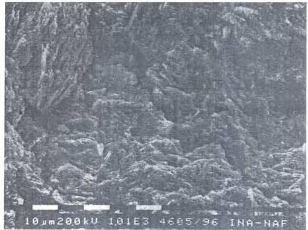
Fig. 6. Surface of spiltized diabase following the fracturing of the sample (bar = 10 μm). Microfractures of this kind are considerably less frequent in diabase compared to andesite, and which are not only of tectonic origin.
