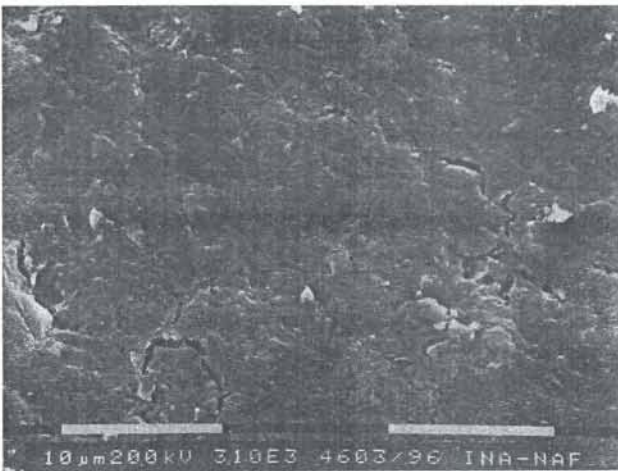
Fig. 5. Surface of spiltized diabase after polishing (bar = 10 μm). Micropores are sparse and sealed, worm-like and bifurcated.
