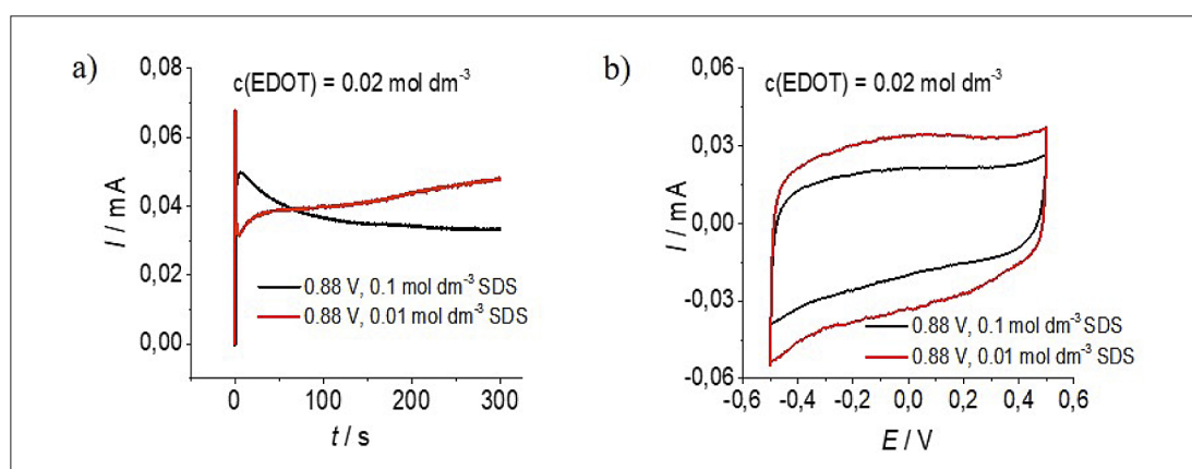
Figure 7: a) Chronoamperometric responses and b) cyclic voltammograms obtained during the synthesis of PEDOT layers in 0.1 \text{ mol dm}^{-3} and 0.01 \text{ mol dm}^{-3} SDS solution during 300 s at 0.88 V; c(\text{EDOT}) = 0.02 \text{ mol dm}^{-3}
