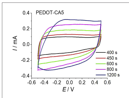
Figure 8: Cyclic voltammograms of PEDOT-CA 5 layer synthesised at different deposition times in 0.1 \text{ mol dm}^{-3} KCl solution; scan rate: 50 \text{ mV s}^{-1}
