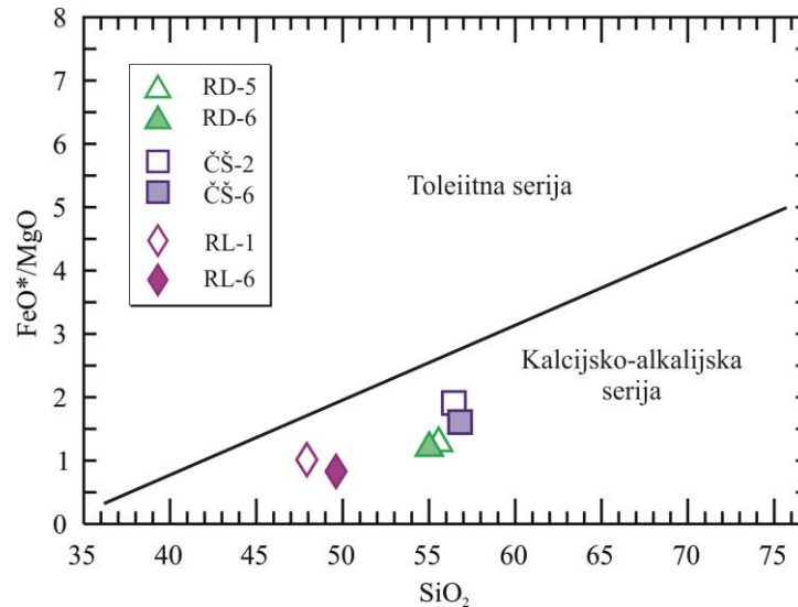
Slika 7-4. Dijagram \text{FeO}^*/\text{MgO}-\text{SiO}_2 prema Miyashiro (1975). Preračunavanje \text{Fe}_2\text{O}_3 u \text{FeO}^* : \text{FeO}^*=0,89981 \times \text{Fe}_2\text{O}_3 .
