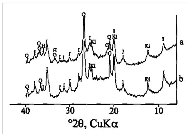
Fig. 2 Characteristic parts of XRD patterns of terra rossa sample 1 (<2 \mu m fraction). Legend: a) air dried; b) treated with HCl (1:1, 24 h); Kl - kaolinite; I - illitic material; Q - quartz; H - haematite; G - goethite.
