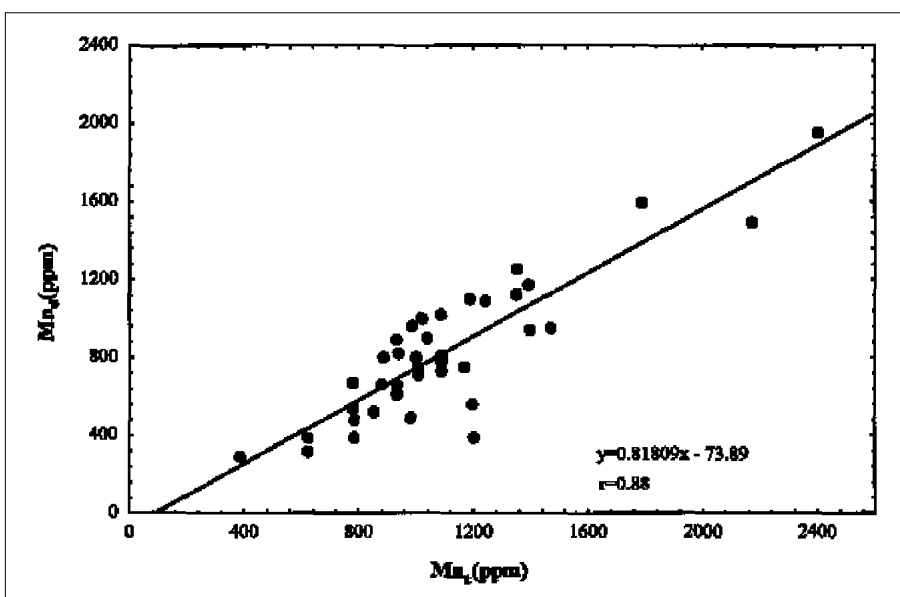
Fig. 8 Ratio between dithionite extractable manganese ( Mn_d ) and total manganese ( Mn_i ) of terra rossa samples; r is significant at the level p < 0.01 .
