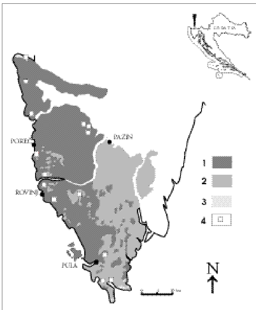
Fig. 1 Distribution of terra rossa in Istria (modified after ŠKORIĆ, 1987). Legend: 1) terra rossa, calcocambisol, eutric cambisol, rigosol from terra rossa (area of terra rossa >70%); 2) terra rossa, calcocambisol, eutric cambisol (area of terra rossa is 50-70%); 3) eutric cambisol on loess, luvisol on loess, rigosol from luvisol and eutric cambisol (40:30:30); (4) location of terra rossa samples.
